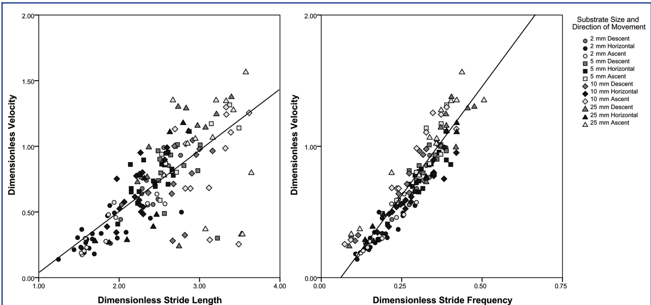
Figure 3. Scatterplot of dimensionless velocity ( V ) first as a function of dimensionless stride length ( SL ) and then as a function of dimensionless stride frequency ( SF ). The regression lines are significant at P < 0.05 , with functions V = 0.43 + 0.47 \times SL (left graph) and V = -0.2 + 3.29 \times SF (right graph).
