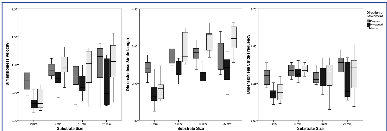
Figure 5. Boxplots of the distribution of dimensionless velocity, dimensionless stride length, and dimensionless stride frequency in the substrate size categories examined, split into three graphs for each direction of movement. The top and bottom sides of the box denote the upper and lower quartiles, the line within the box is the median, while the top and bottom whiskers represent the maximum and minimum values obtained.
